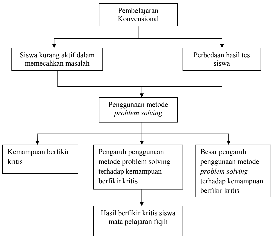
Gambar 2.1 Paradigma Penelitian
