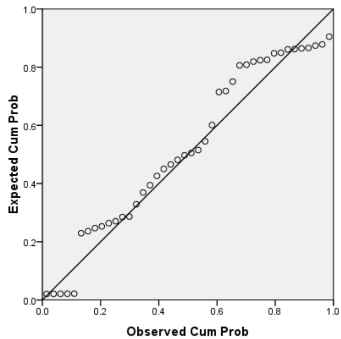
Normal P-P Plot of LIKUIDITAS BANK MEGA SYARIAH
