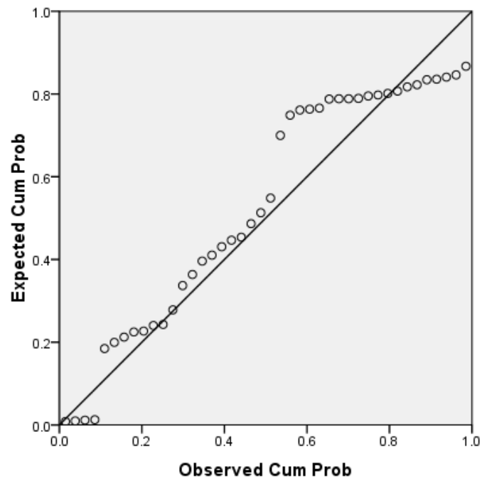
Normal P-P Plot of DPK
