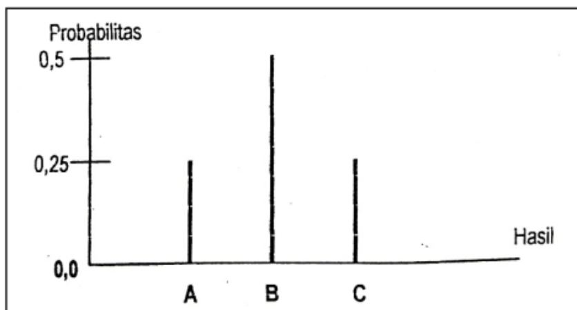
Gambar 4.6 Kurva Probabilitas
