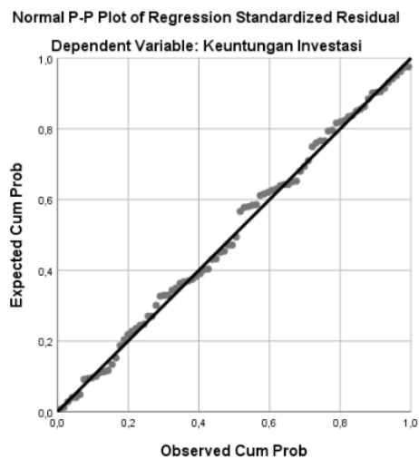
Gambar. 2 P-P Plot
