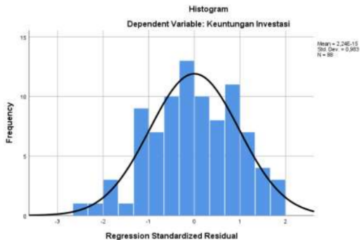
Gambar. 1 Histogram
