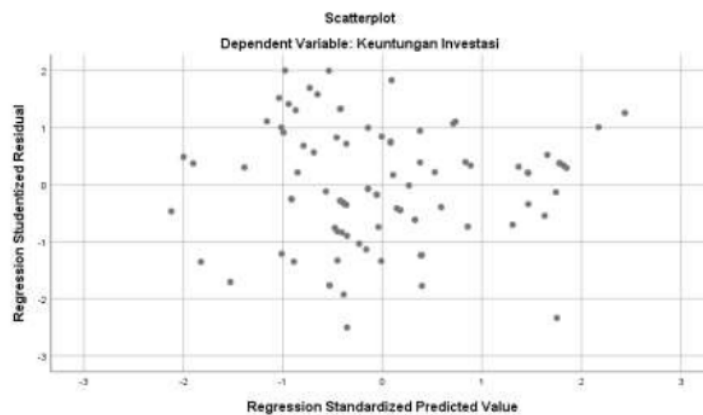
Gambar. 3 Scatterplot
