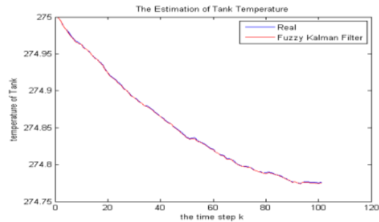
Fig. 3. The FKF estimation of Temperature Tank, T
