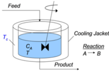
Fig. 1. Nonisothermal Continuous Stirred Tank Reactor [11]
