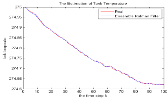
1 Fig. 6. The EnKF estimation of Temperature Tank, T
