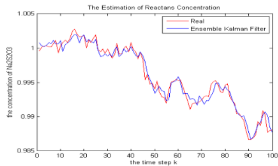
Fig. 5. The EnKF estimation of Concentration Reactance, C_A
